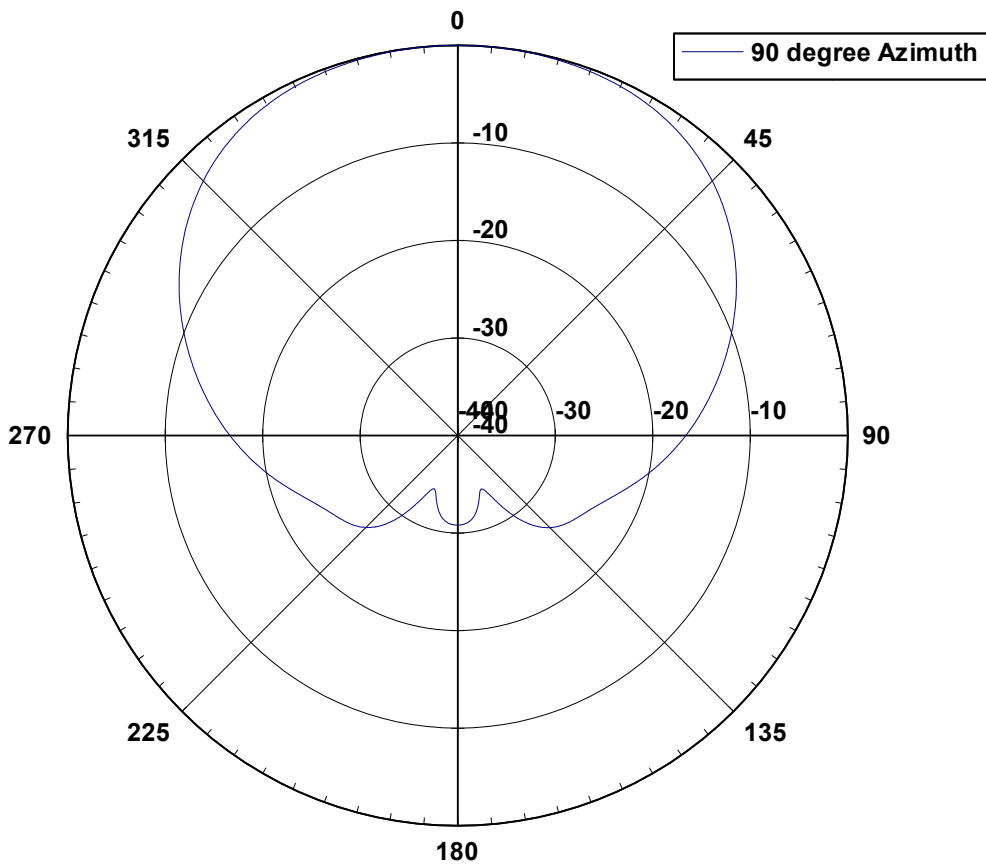
26 9010 Elevation Pattern
