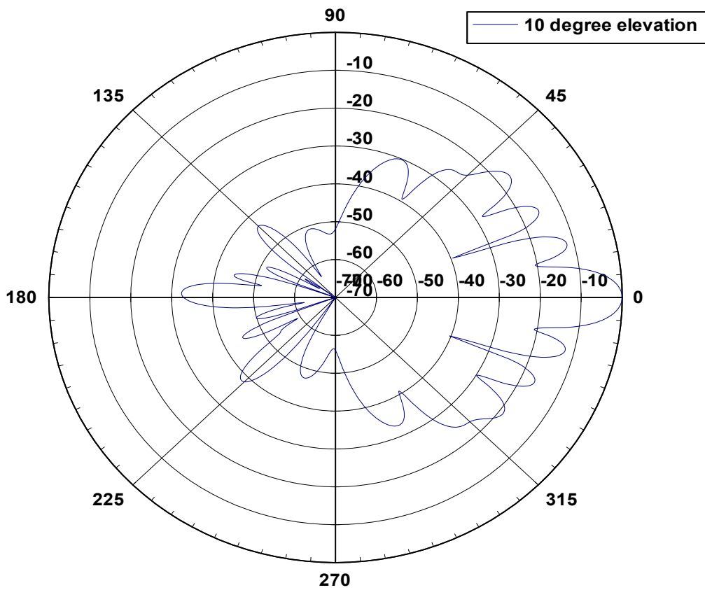
26 9010 Elevation Pattern
