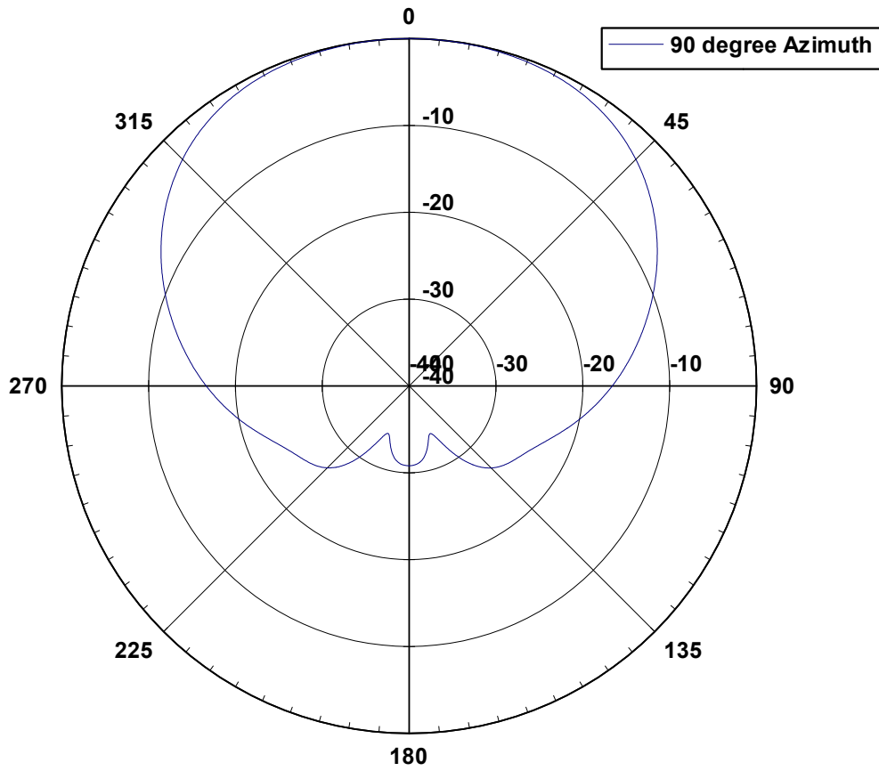
26 9007 Elevation Pattern
