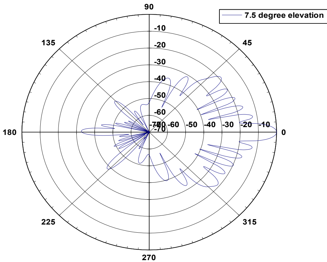
26 9007 Elevation Pattern
