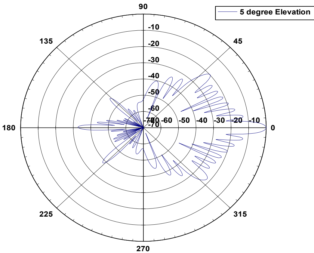
26 9005 Elevation Pattern
