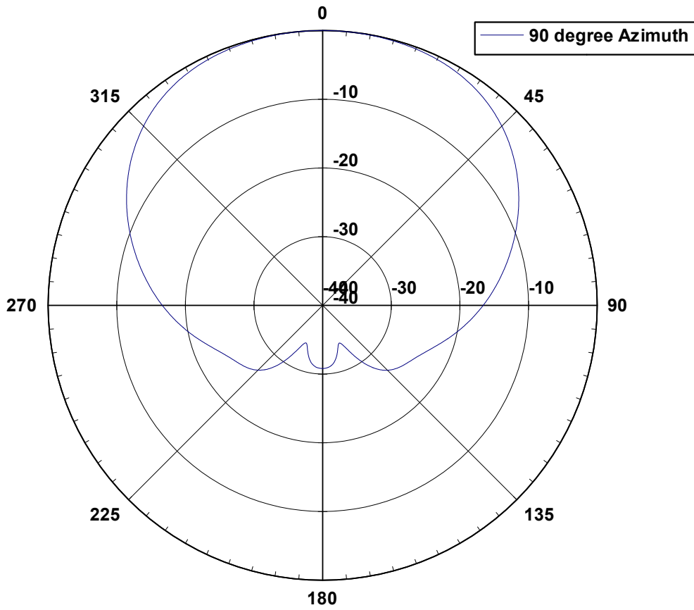
26 9005 Elevation Pattern
