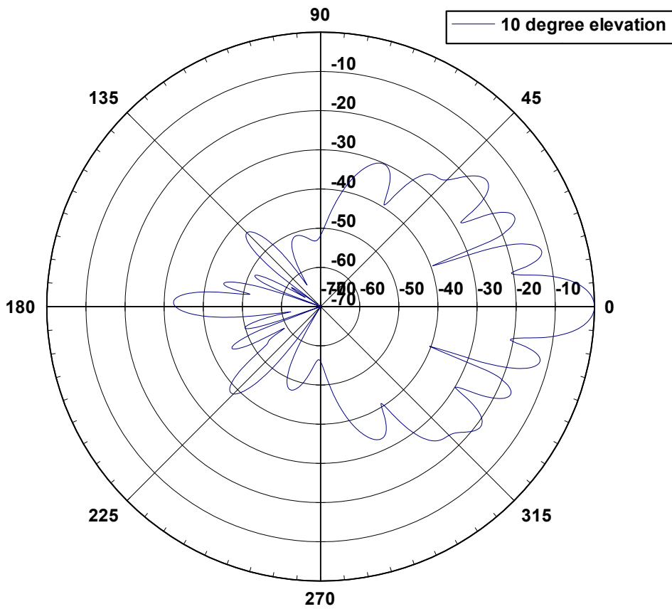
26 6010H Elevation Pattern
