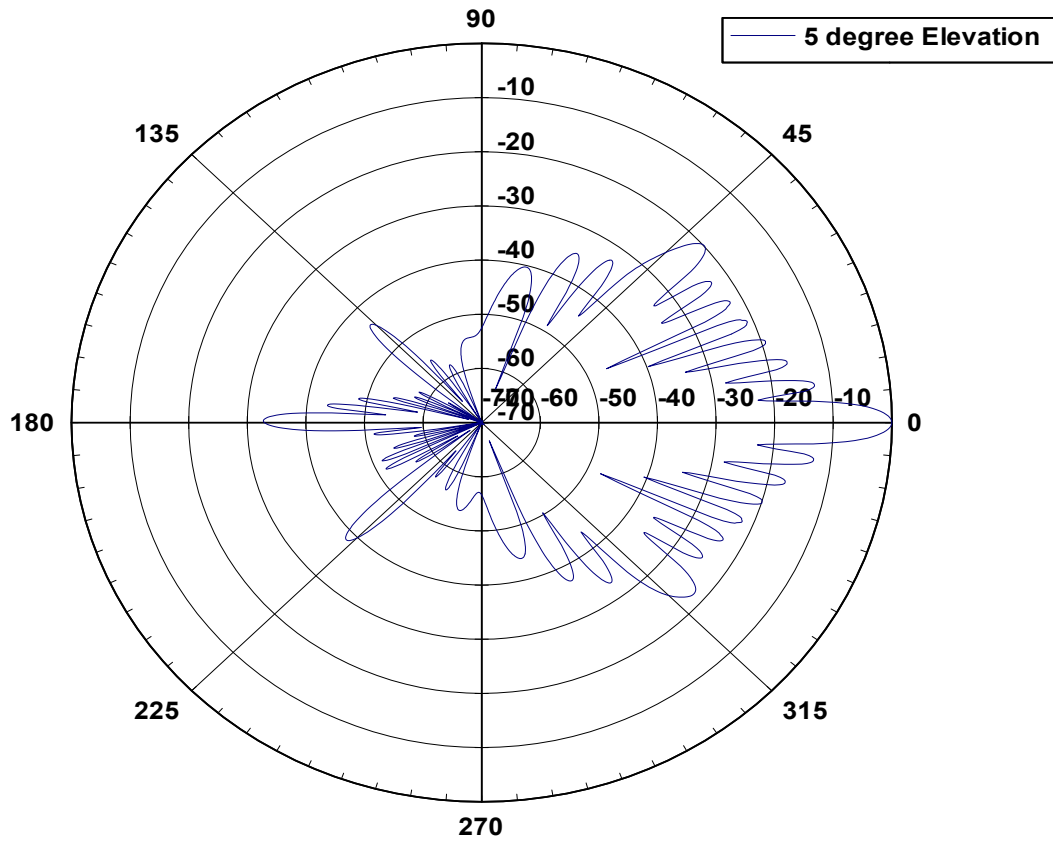
26 6005H Elevation Pattern
