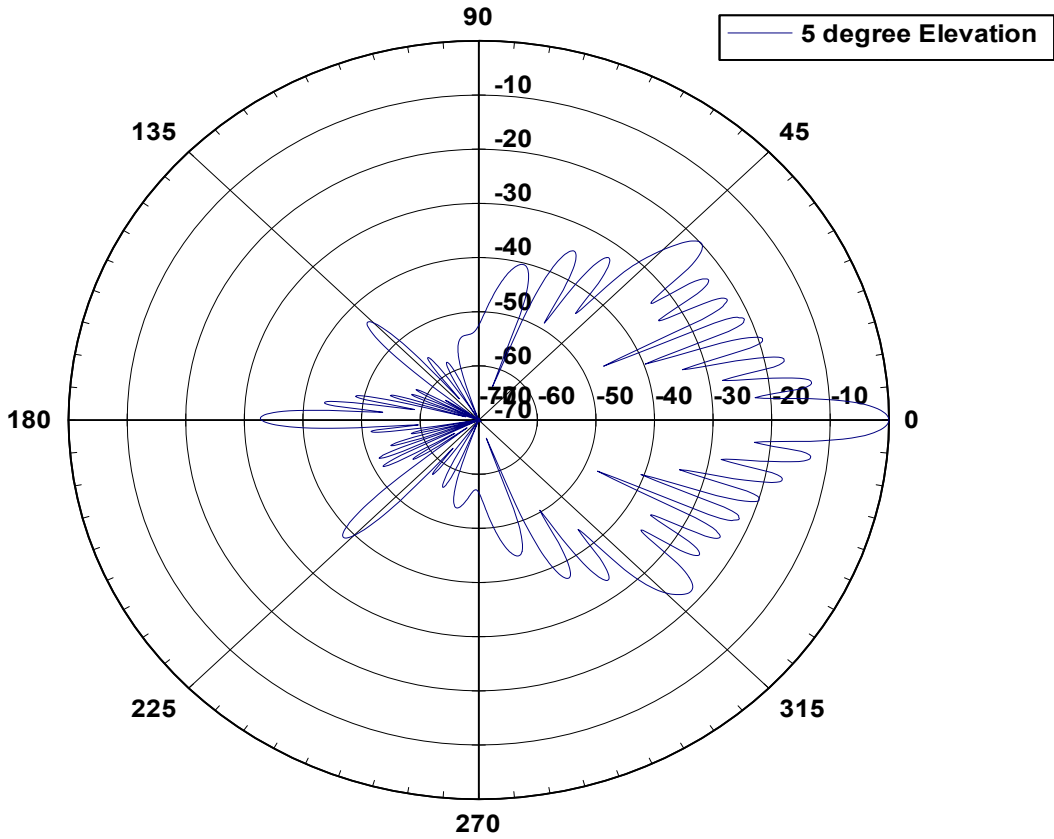
26 6005 Elevation Pattern
