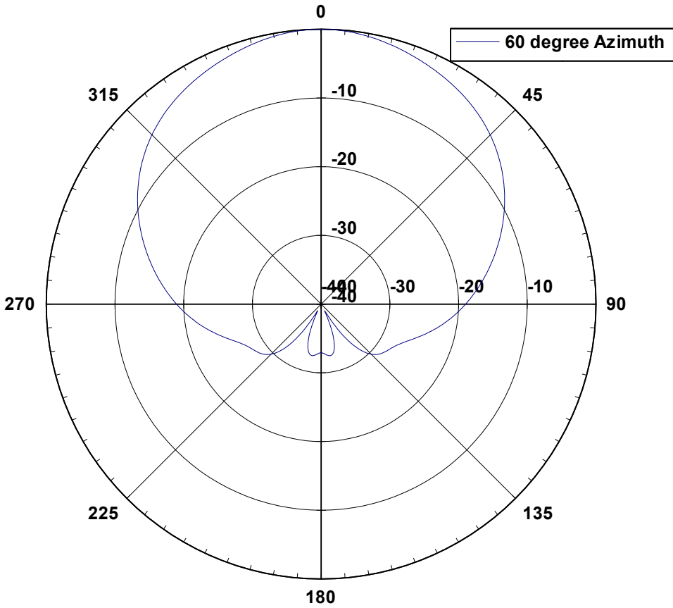
26 6005 Elevation Pattern
