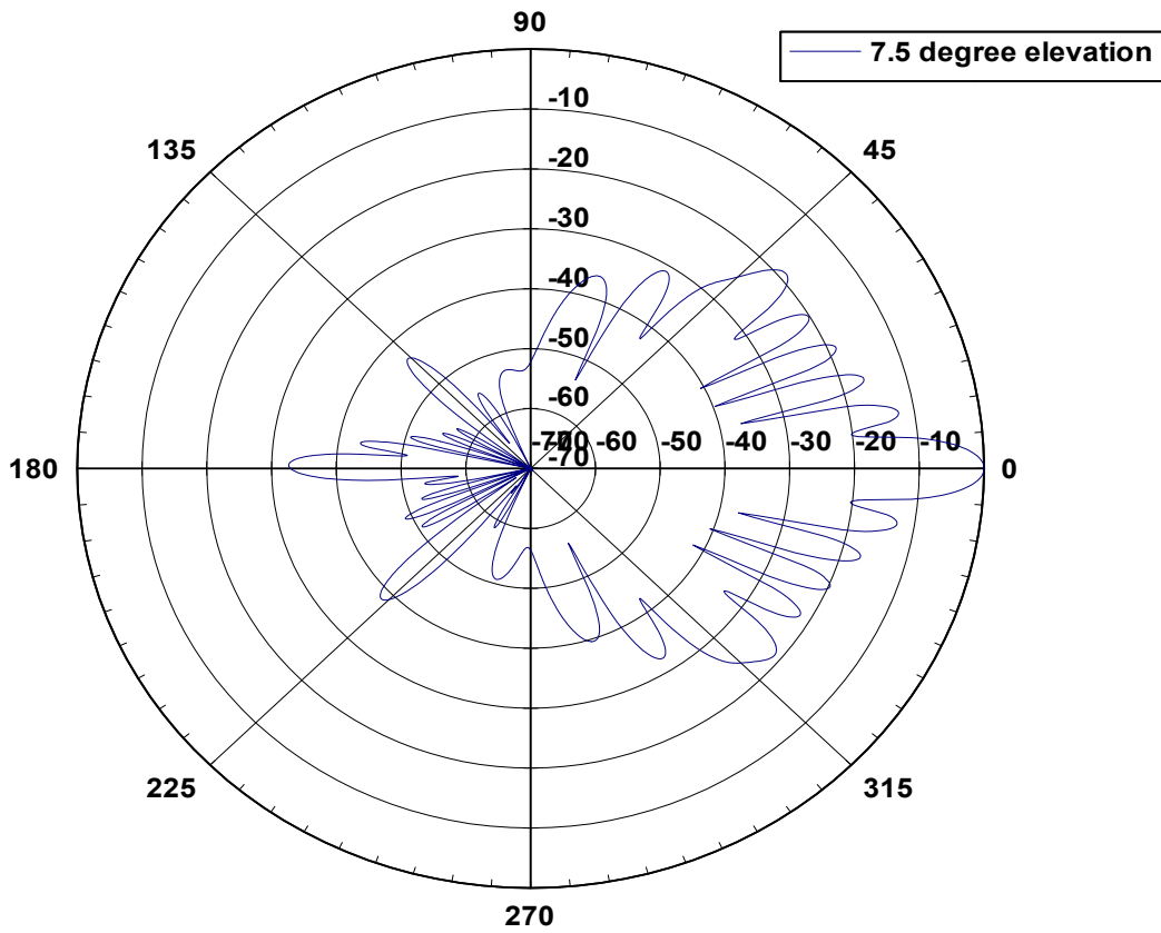
26 4507 Elevation Pattern
