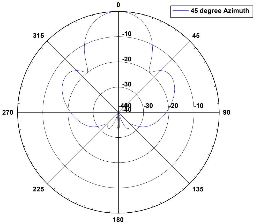
26 4505H Elevation Pattern
