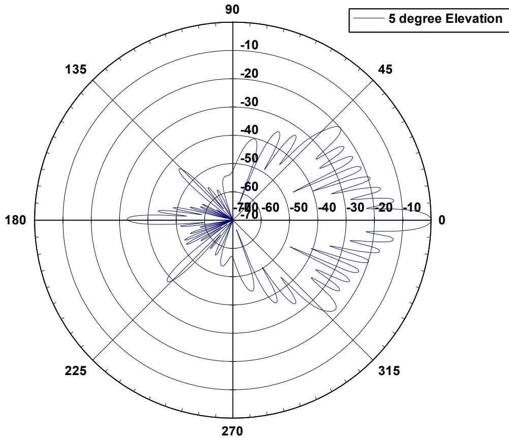
26 4505H Elevation Pattern
