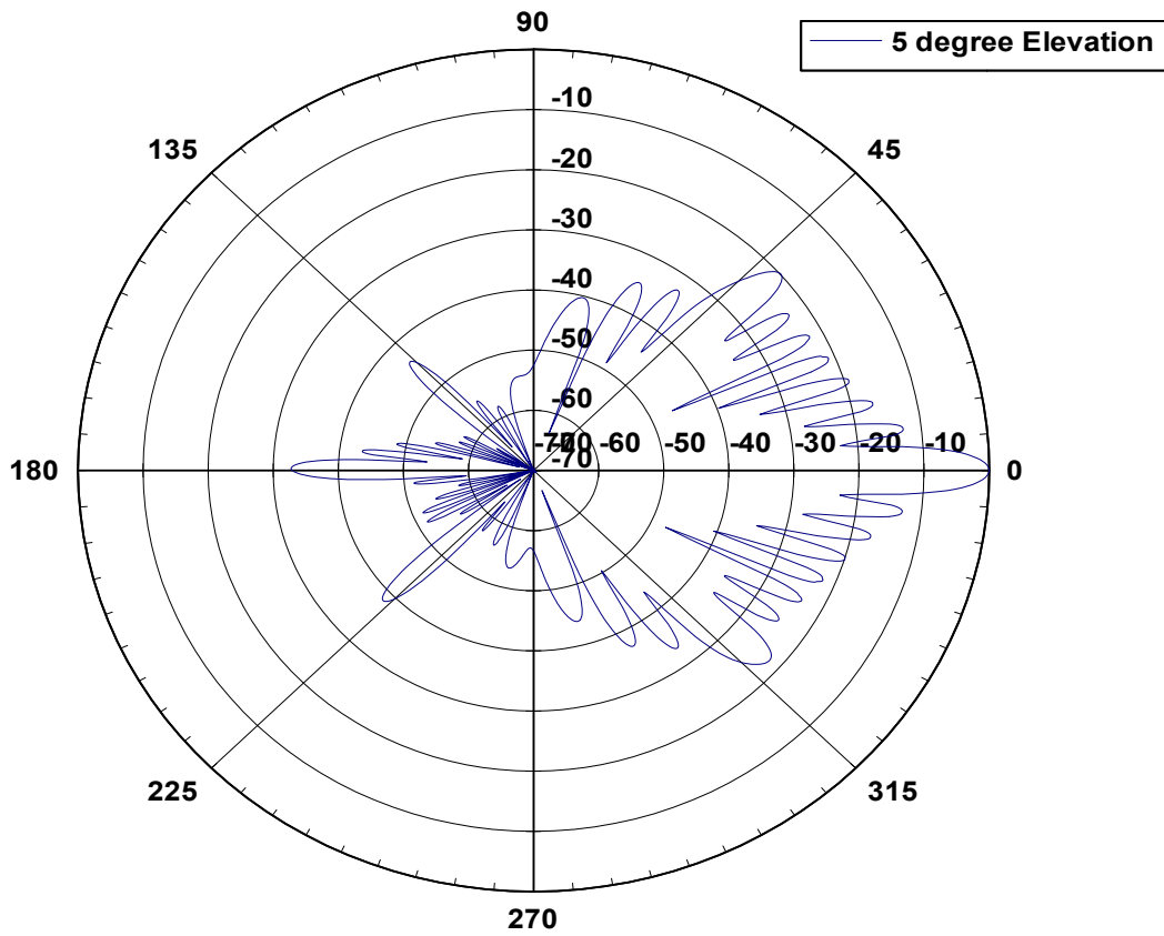
26 4505 Elevation Pattern
