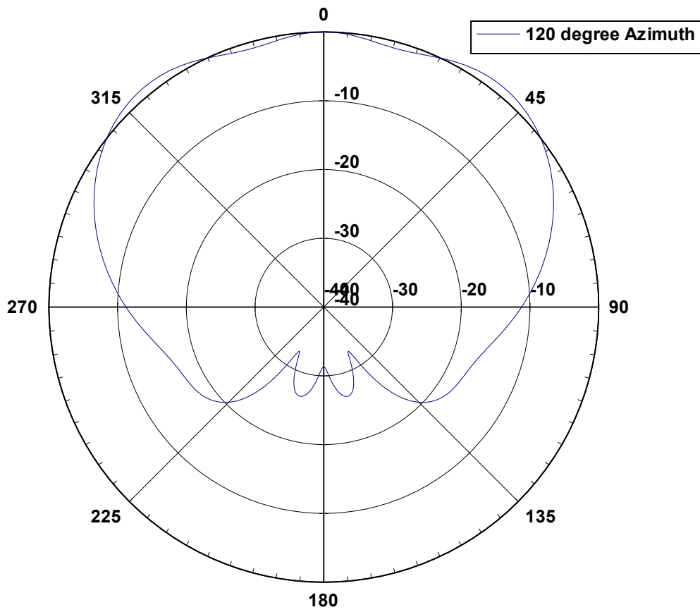
26 12005 Elevation Pattern
