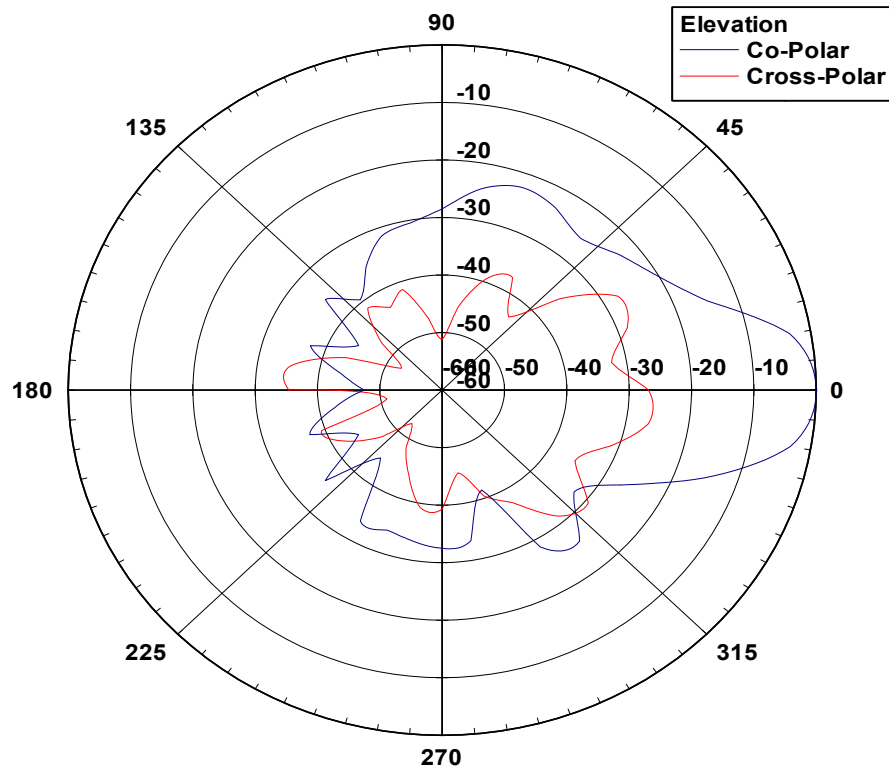
Elevation Pattern
