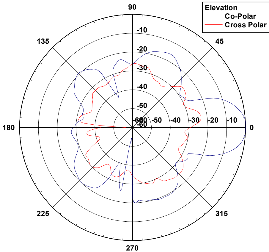
26 SD15 Elevation Pattern
