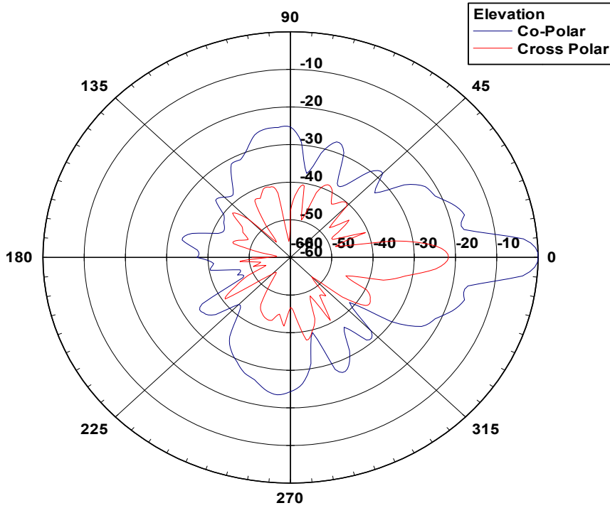
22 SD27 Elevation Pattern
