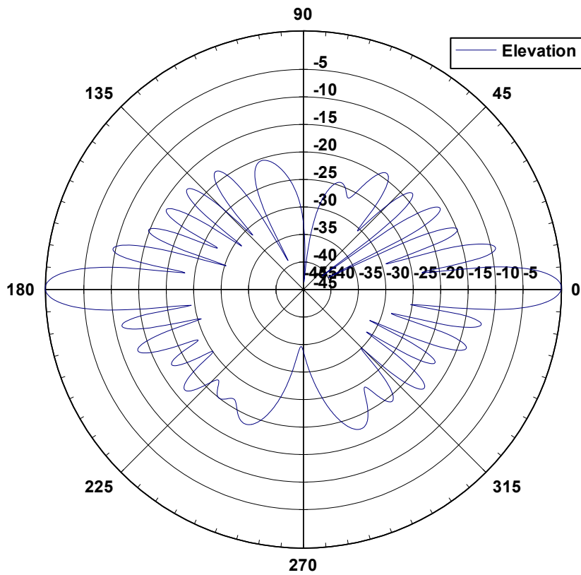
26 2360 Elevation Pattern
