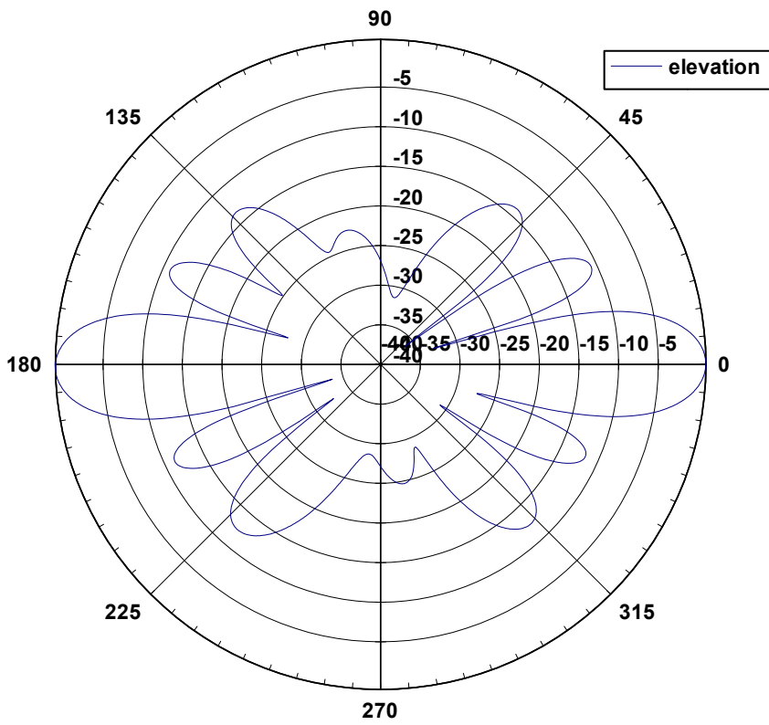
26 1360 Elevation Pattern
