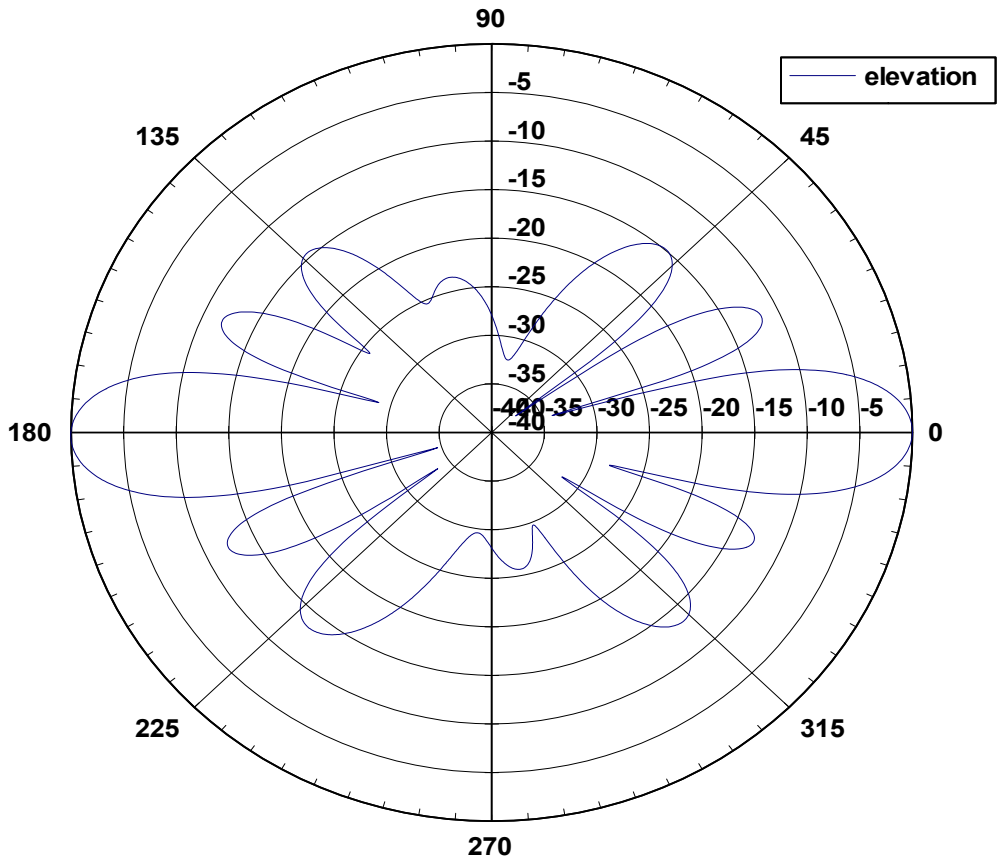
22 1360 Elevation Pattern
