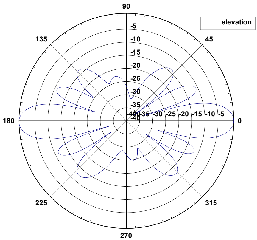
22 1360 Elevation Pattern
