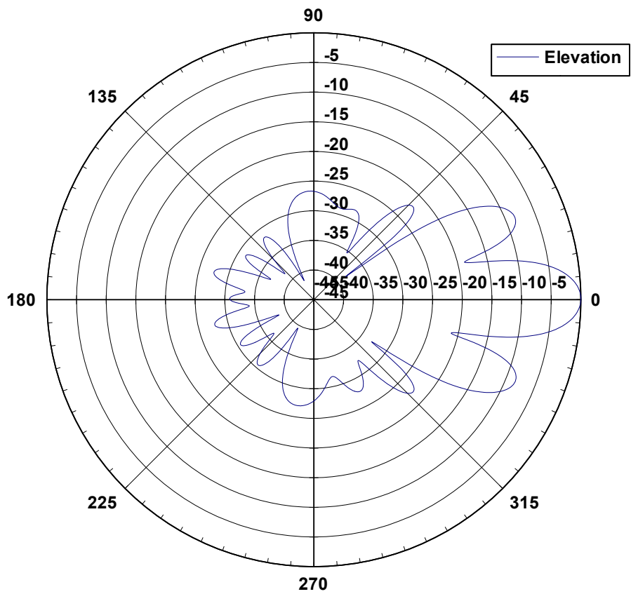
26 9015 Elevation Pattern
