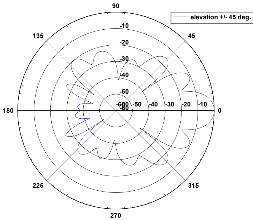
26 6015 XP Elevation Pattern
