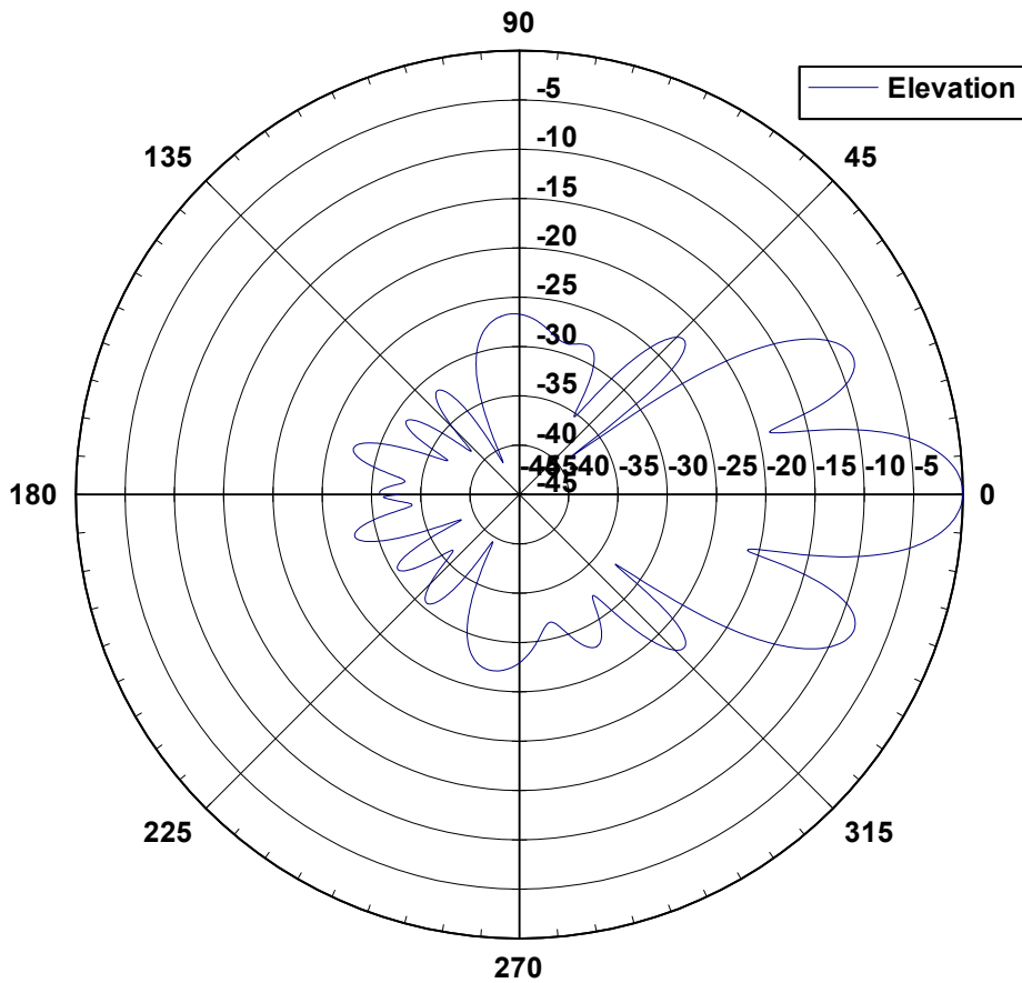
26 6015 Elevation Pattern
