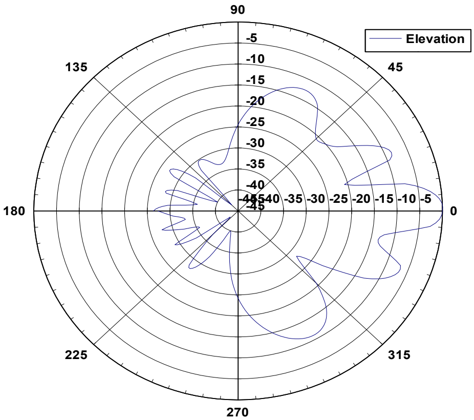
26 3015 Elevation Pattern
