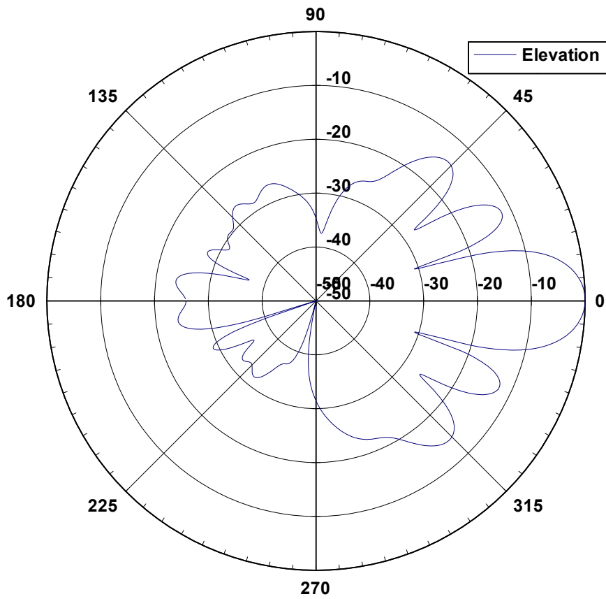
26 18015 Elevation Pattern
