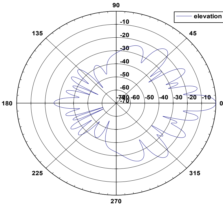
26 12008 Elevation Pattern
