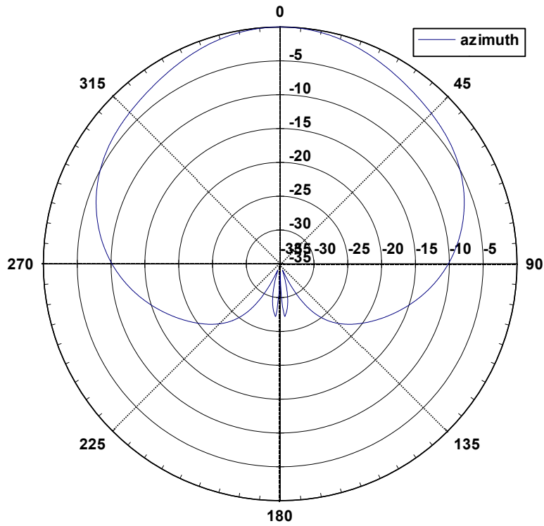
Azimuth Pattern
