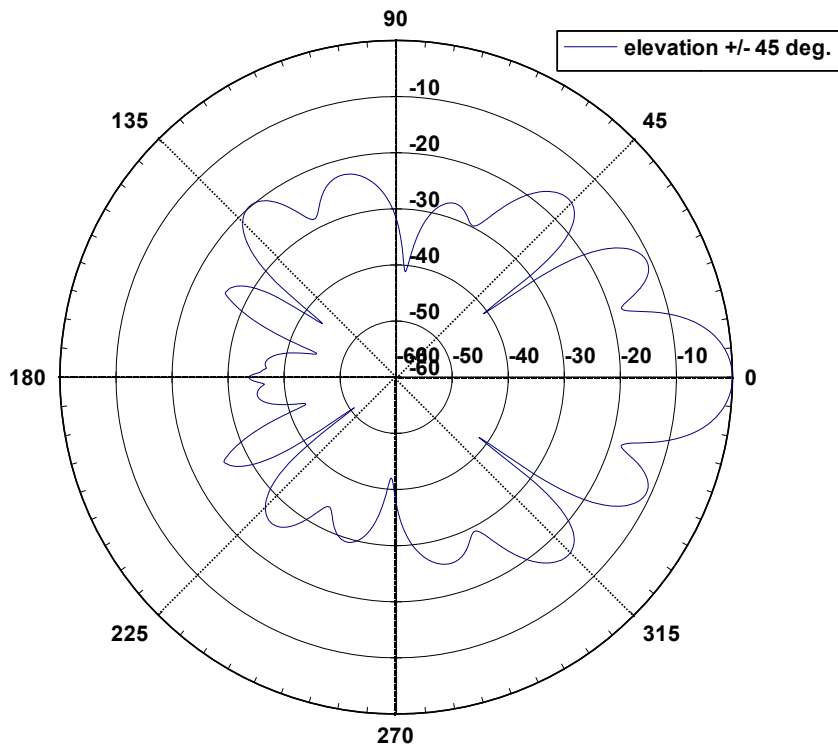
Elevation Pattern
