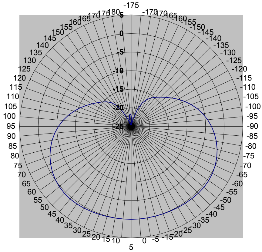
26 18008 13dBi Base Station Azimuth Pattern
