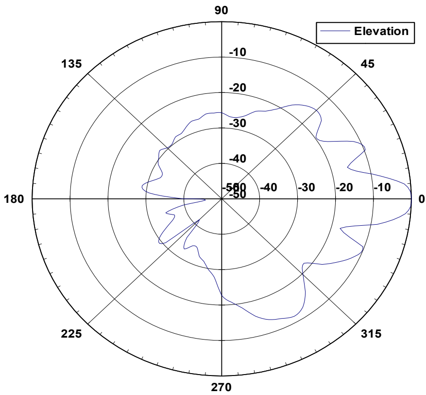
22 9015 Elevation Pattern
