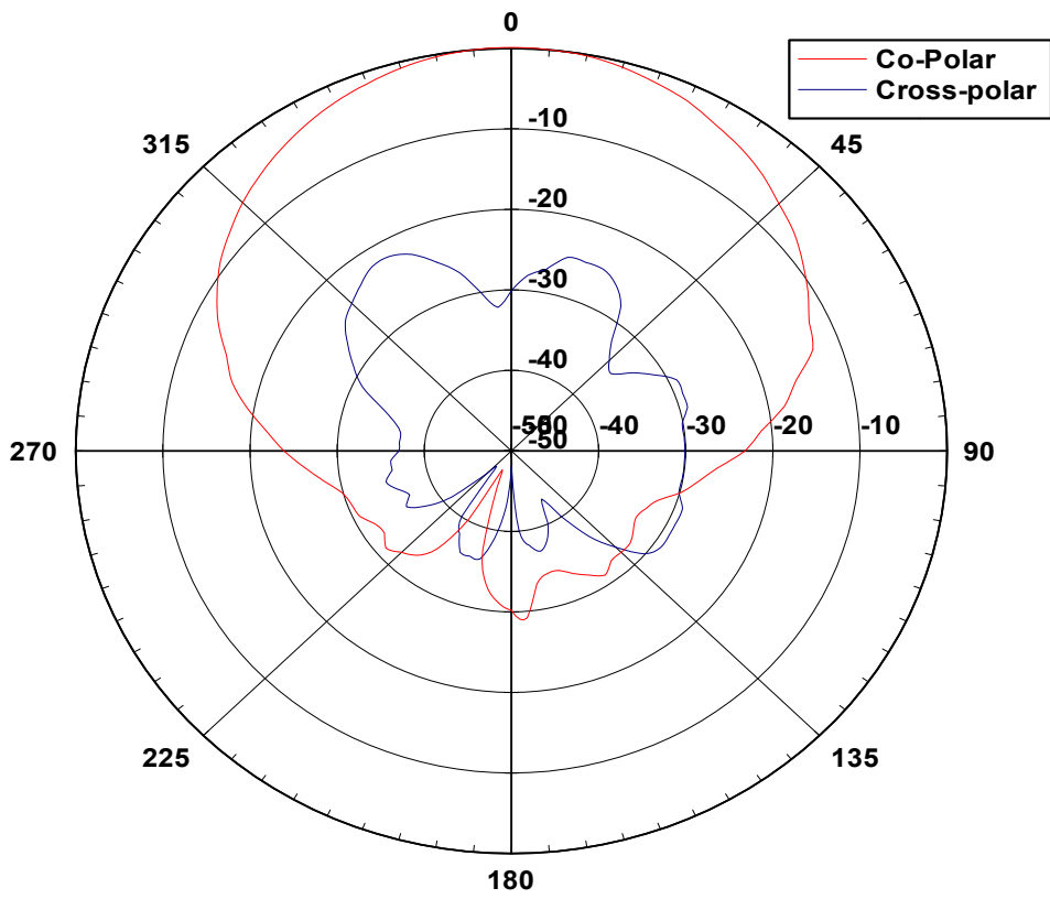
22 6008H Elevation Pattern
