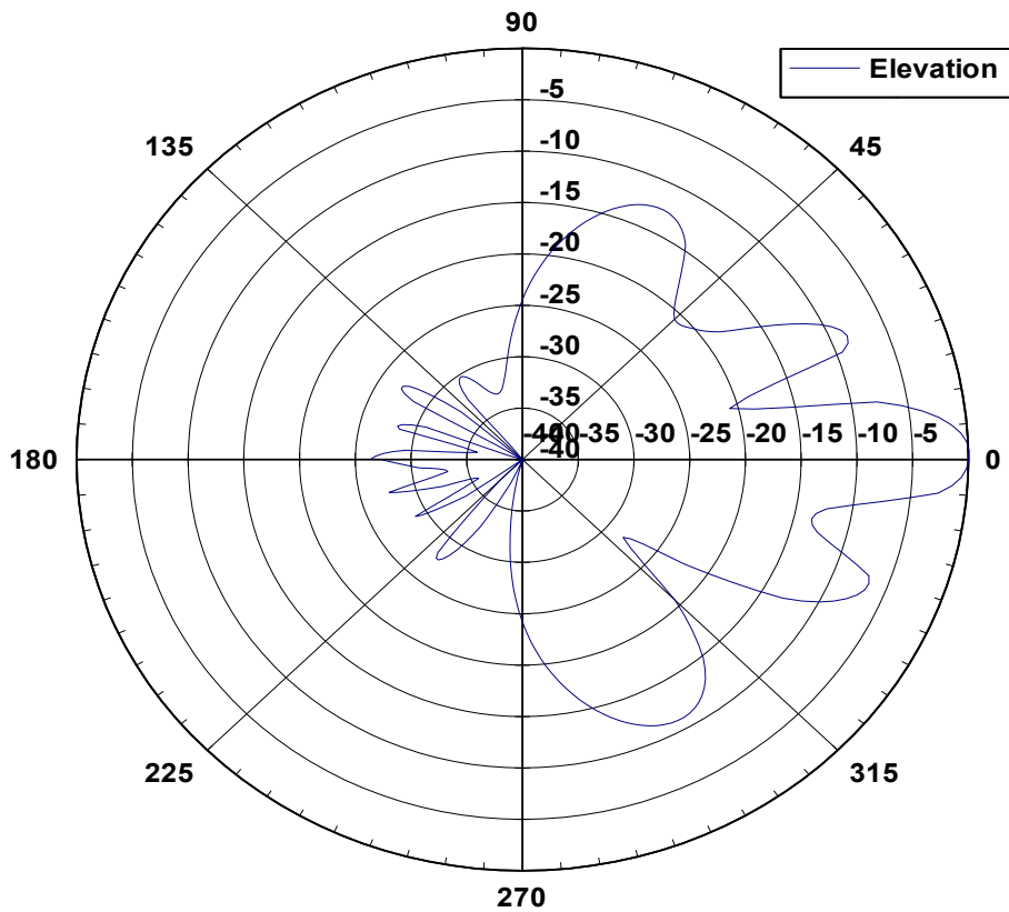
22 3105 Elevation Pattern
