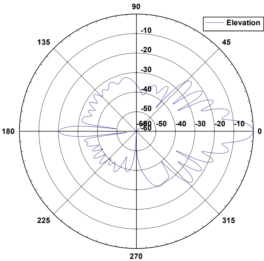
22 18008 Elevation Pattern
