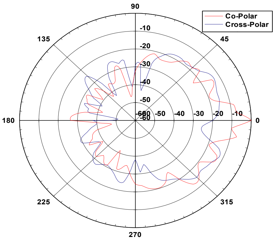
22 12008 Elevation Pattern
