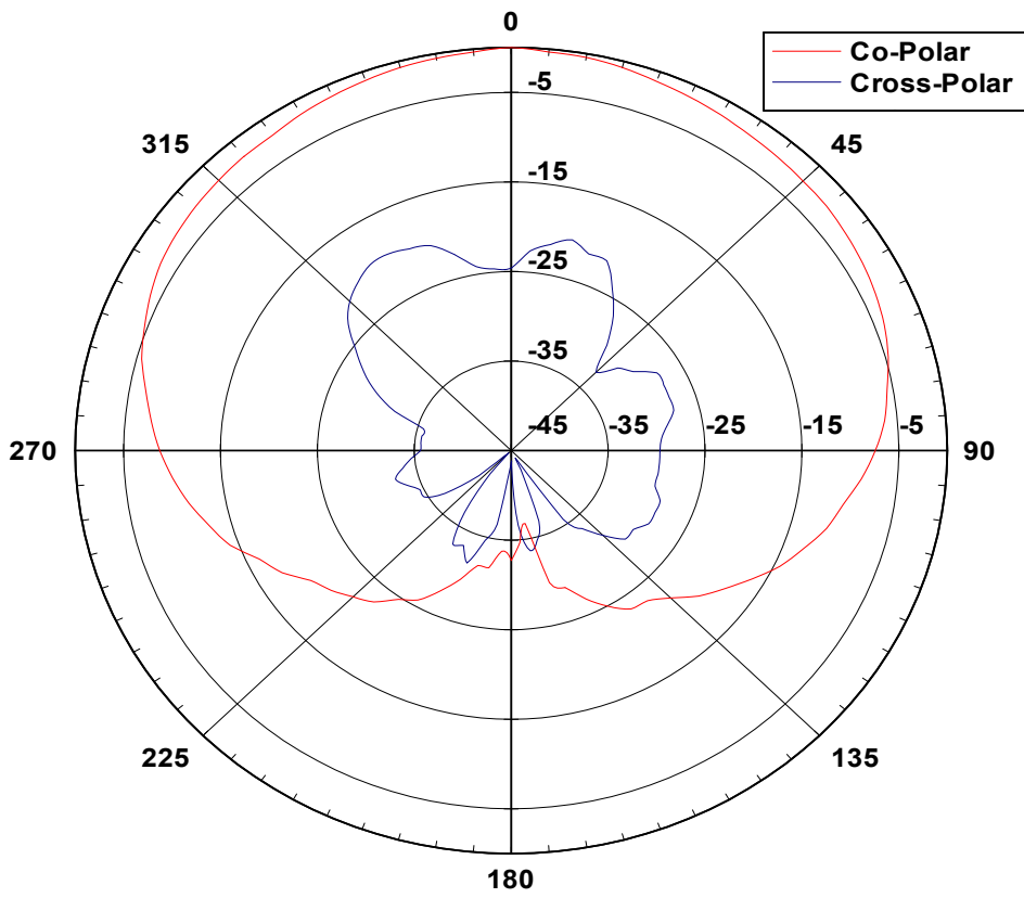
22 12008 Elevation Pattern
