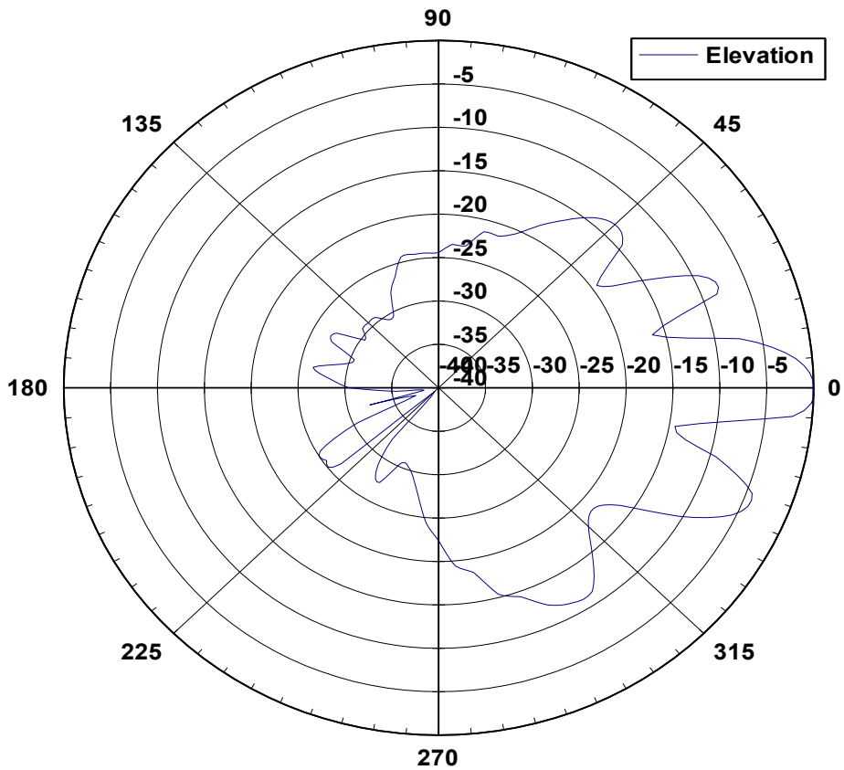
22 12015 Elevation Pattern
