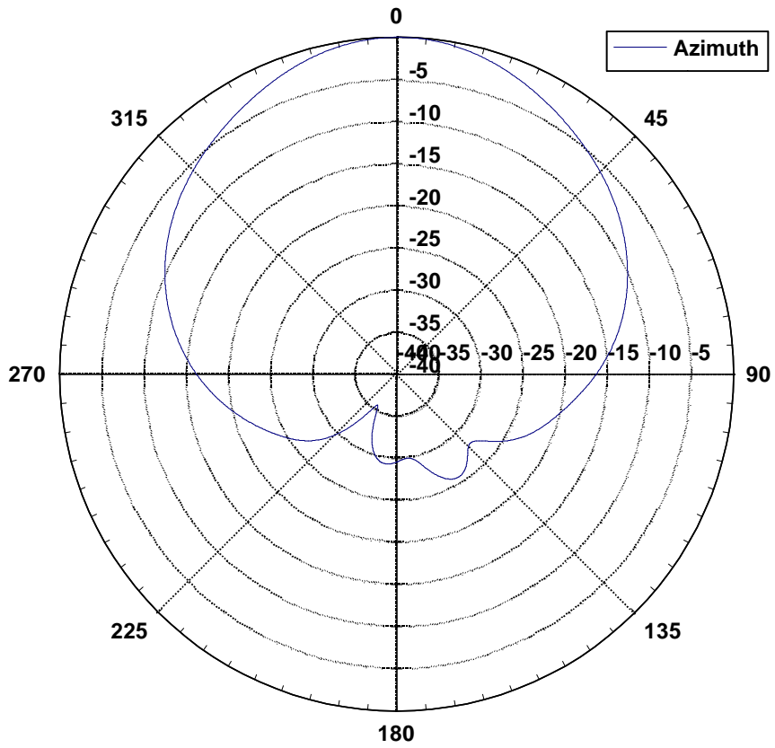
Azimuth Pattern
