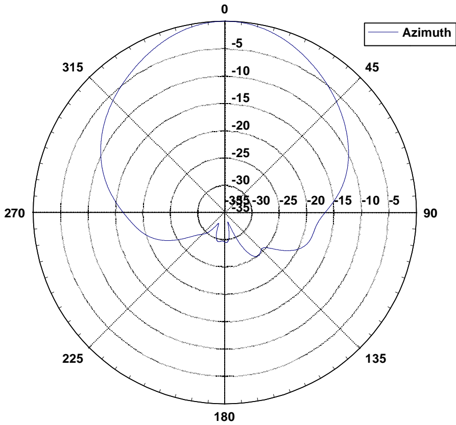
Azimuth Pattern
