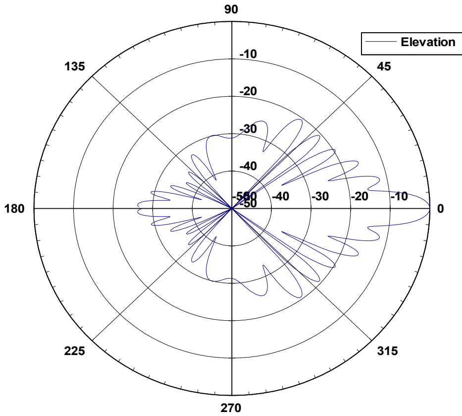
33 SD98120NV Elevation Pattern
