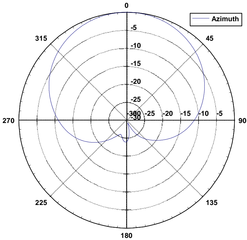
Azimuth Pattern
