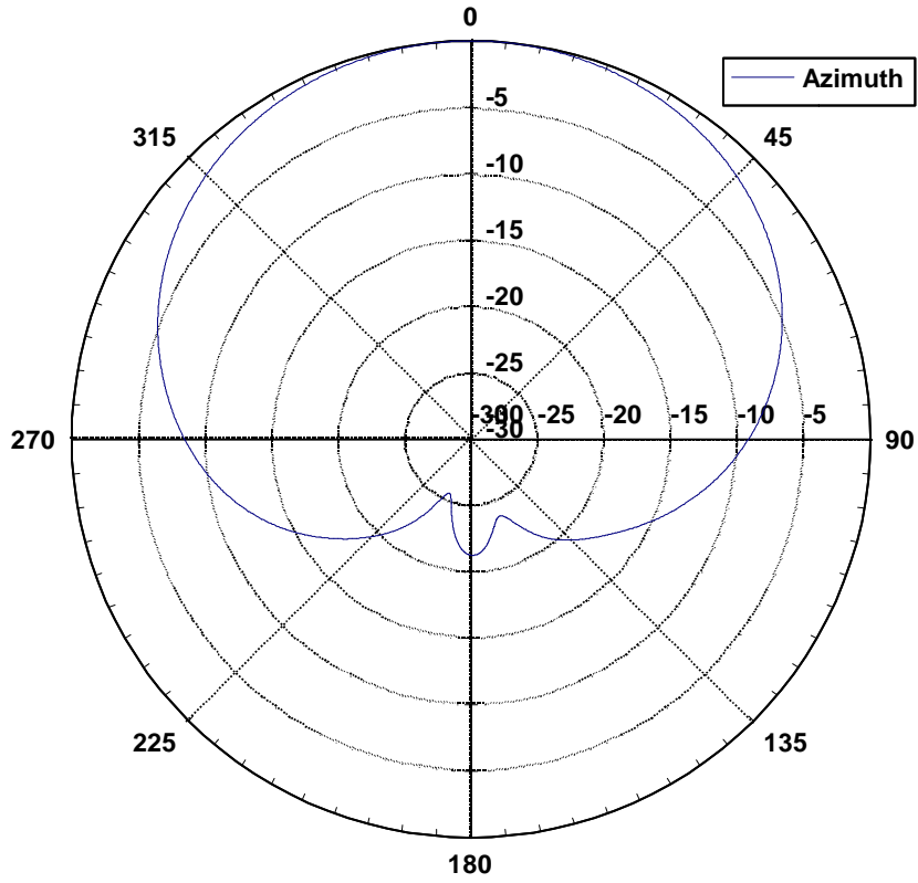
Azimuth Pattern
