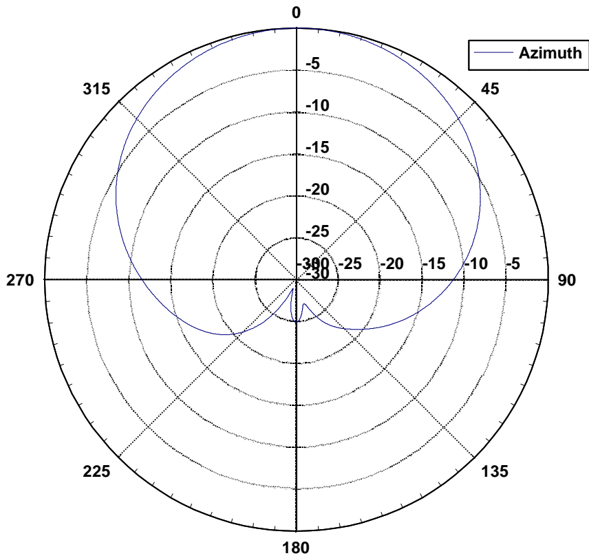
Azimuth Pattern
