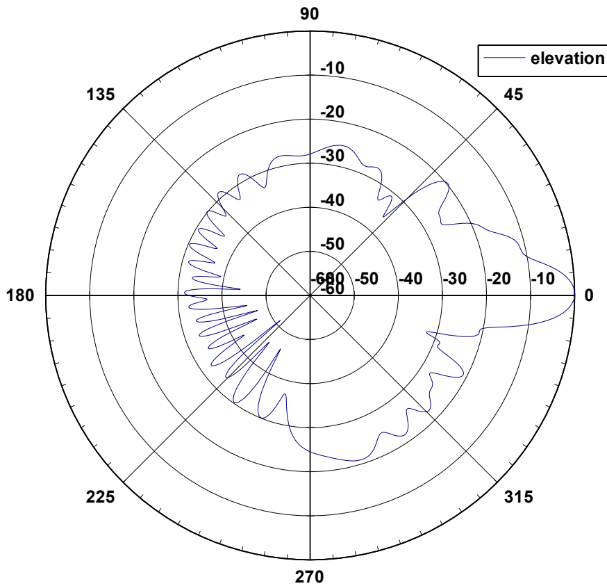
26 SD9860NV-SUS 1 Elevation Pattern
