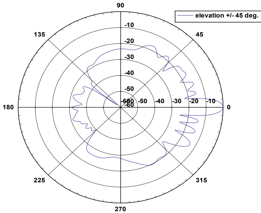
35 9008 XP-MIMO Elevation Pattern
