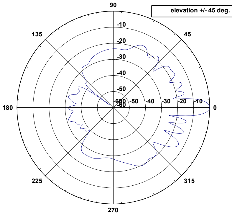
26 9008 XP XP MIMO Elevation Pattern
