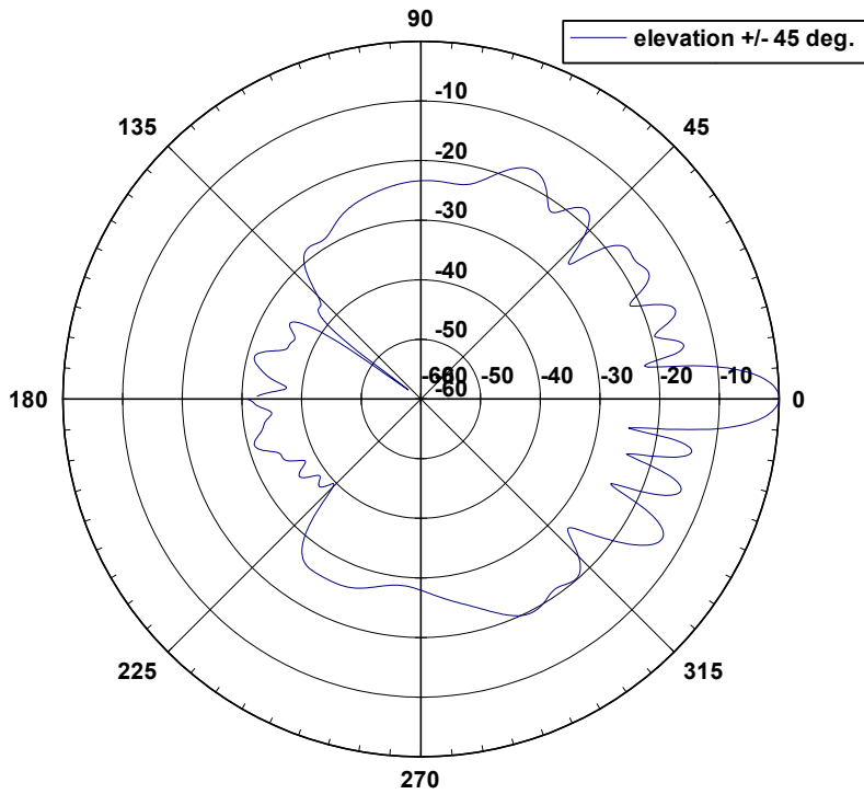
26 9008 XP Elevation Pattern
