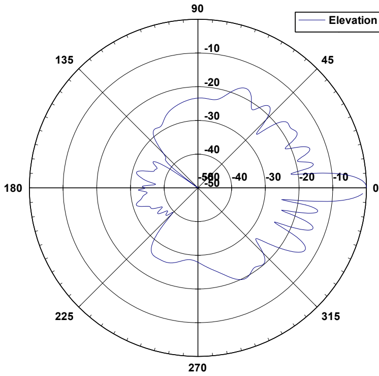
26 6008 XP Elevation Pattern
