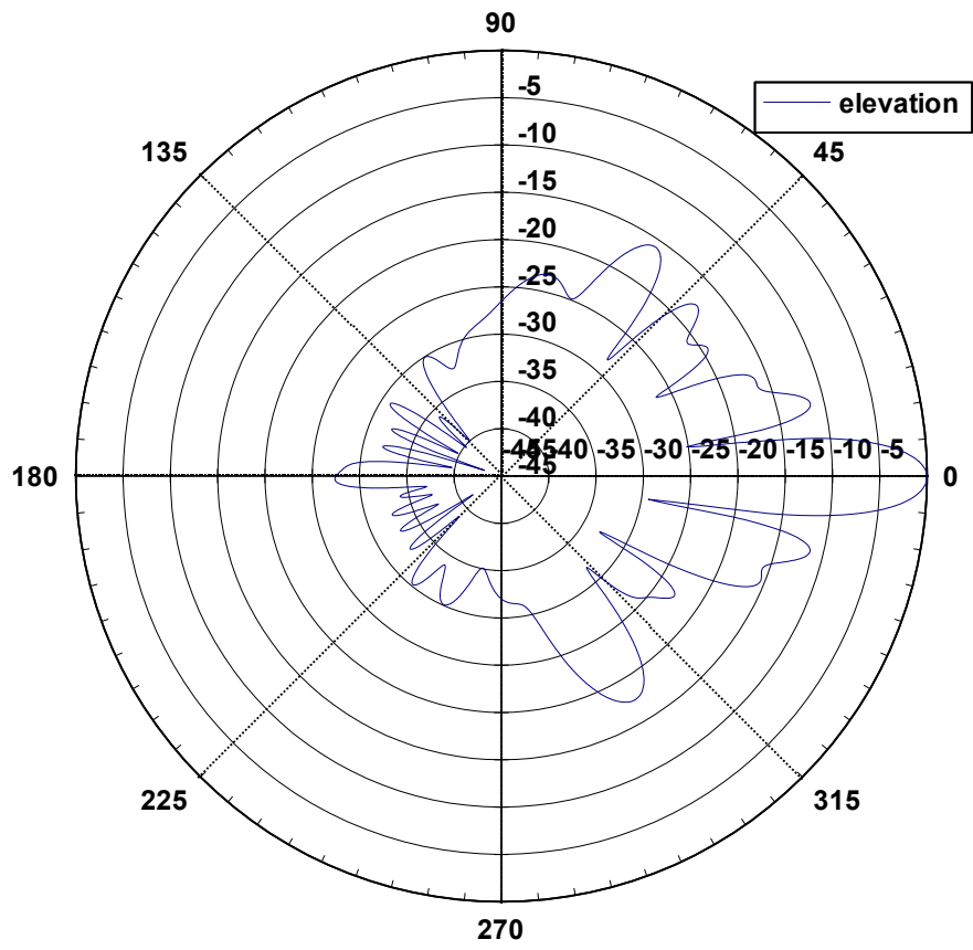
58 9010H Elevation Pattern
