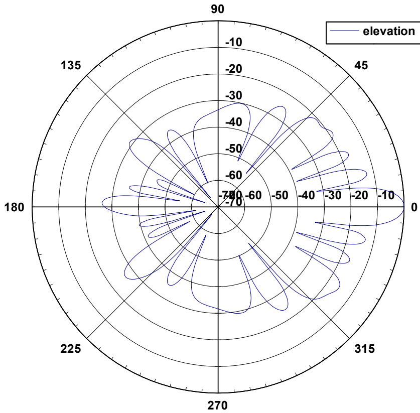
58 6010H Elevation Pattern
