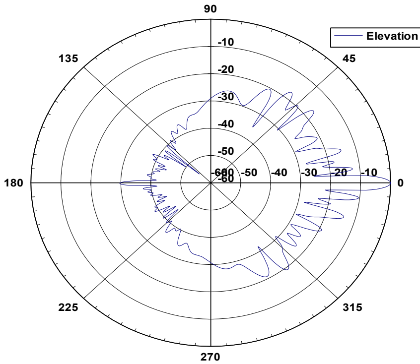
58 6004H Elevation Pattern
