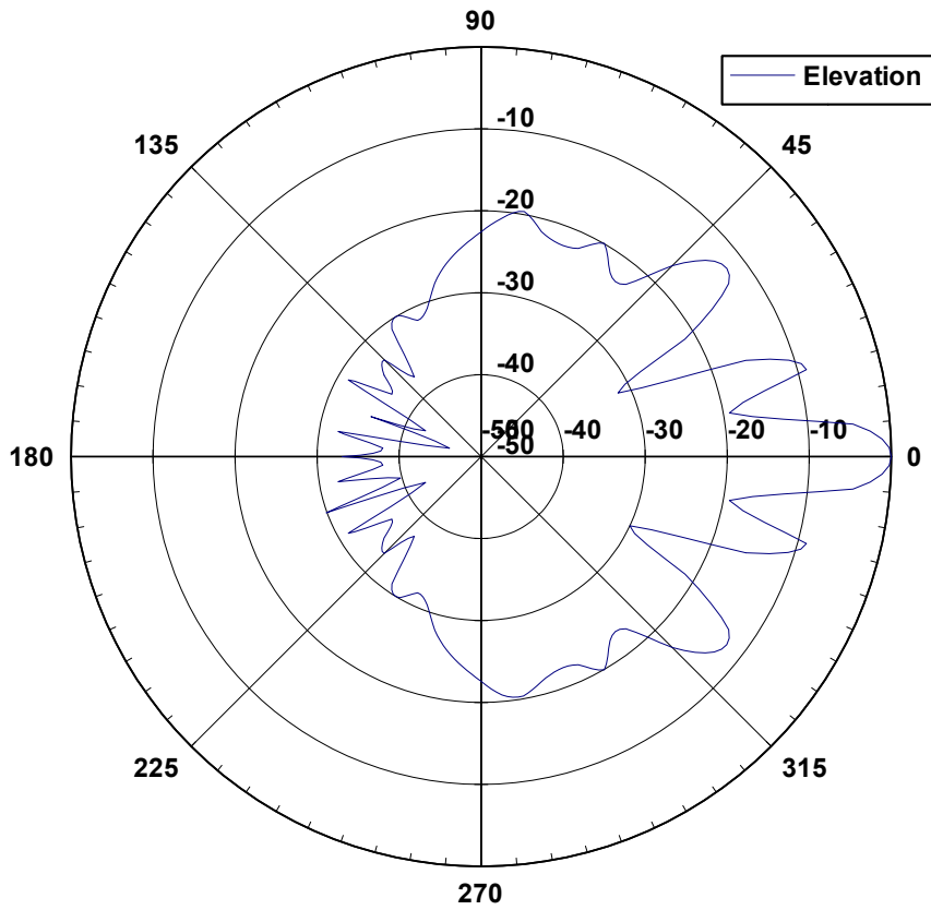
58 3010 Elevation Pattern
