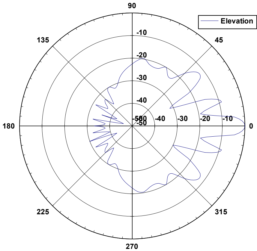
58 3010 Elevation Pattern
