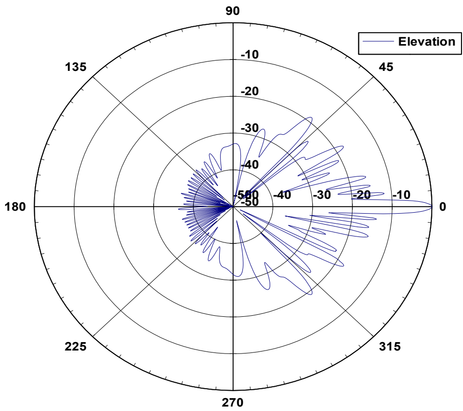
58 3004 Elevation Pattern
