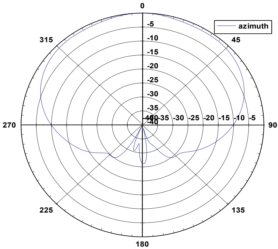
58 12010 Azimuth Pattern
