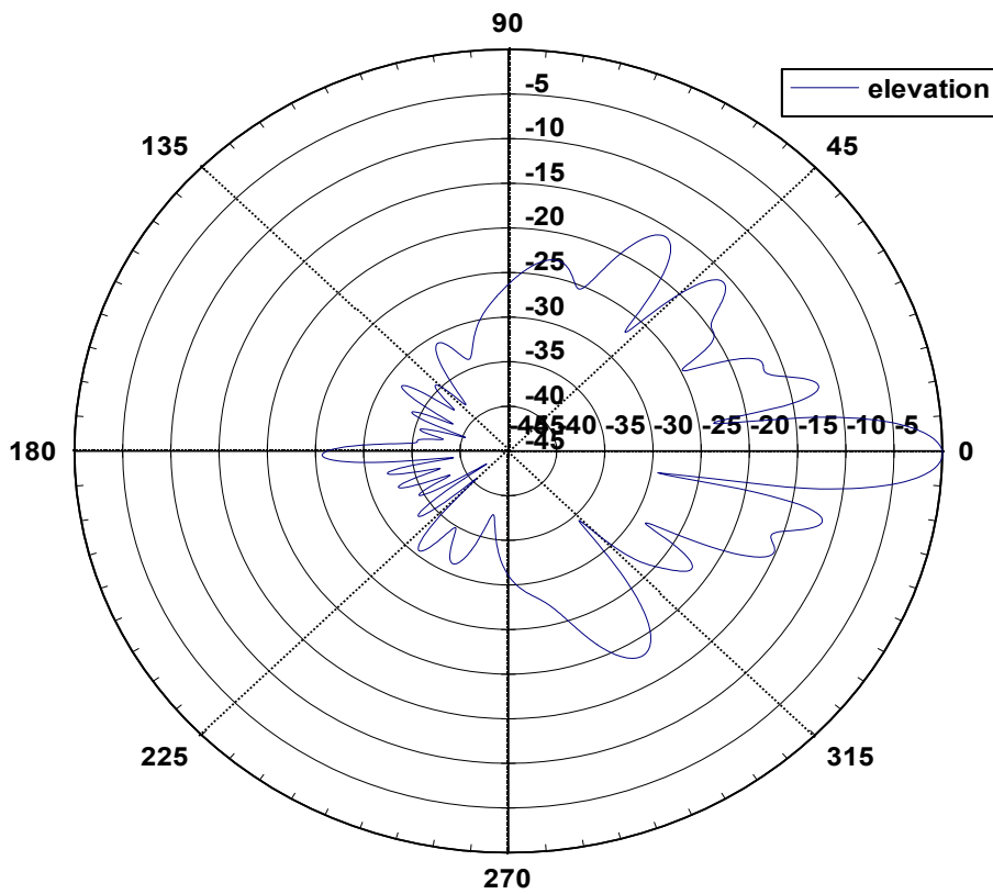
58 12010 Elevation Pattern
