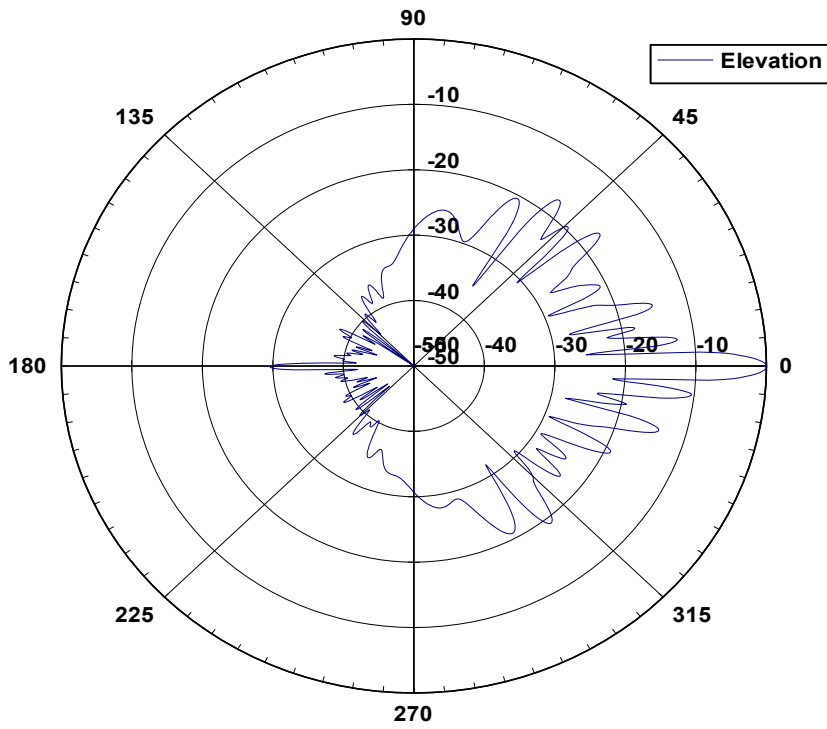
58 12004 Elevation Pattern
