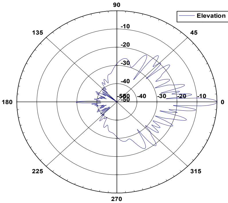
56 9004H Elevation Pattern
